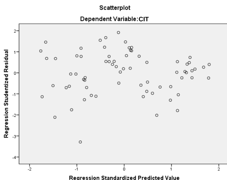
Figure 4. Heteroscedasticity Model 2
